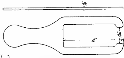
BEARING-THICKNESS GAUGE 3 3/4 x 7 & 4 1/2 x 8 JOURNALS
